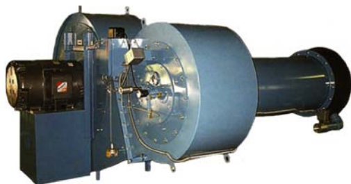
WEBSTER HDR-RF Series Burners Register Burners Model HDR-RF For Water Tube Boilers above 900 BHP Fire Tube Boilers above 1,000 BHP Burner Input 10 MMBtu/Hr 200 MMBtu/Hr Gas Burners/Oil Burners Combination/Low NOx
